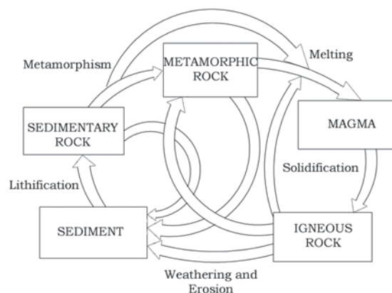
Fig 5.1 : Rock Cycle
