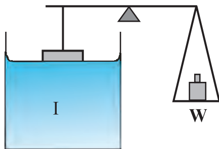
Fig. 10.18 Measuring Surface Tension.
